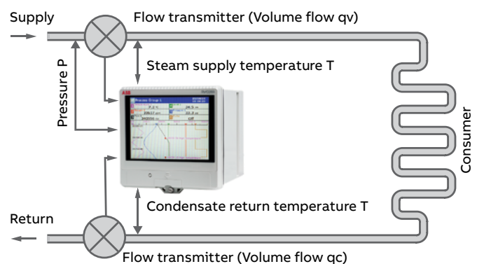
07 Steam power balance energy equation
