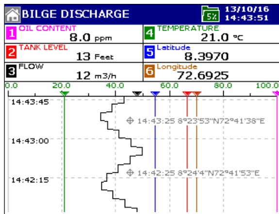
04 Bilge water discharge monitoring window
