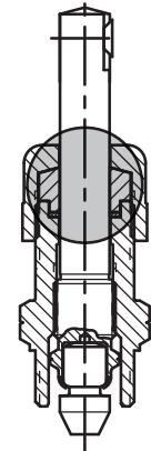
TFE Packing (6801L8Y only)
