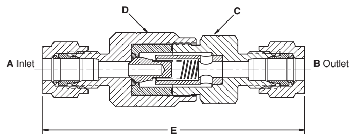
6200 Series Poppet Check Valves
