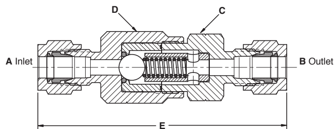
6100 Series Ball Check Valves
