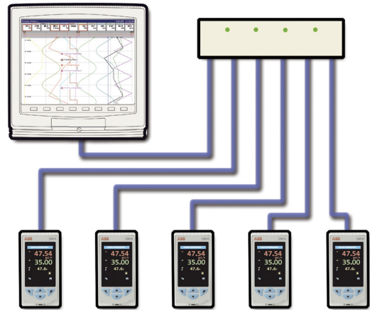
Fig. 11: ControlMasters connected to a ScreenMaster
