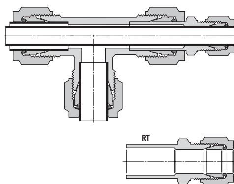
Assembly of Tee Union Tees With Full Port Reducer
